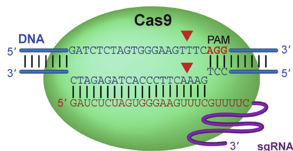
Figure 1. The CRISPR-Cas9 system. The sgRNA (purple) targets the Cas9 protein to genomic sites containing sequences complementary to the 5' end of the sgRNA. The target DNA sequence needs to be followed by a proto-spacer adjacent motif (PAM), typically NGG. Cas9 is a DNA endonuclease with two active domains (red triangles) cleaving each of the two DNA strands three nucleotides upstream of the PAM. The five nucleotides upstream of the PAM are defined as the seed region for target recognition.
