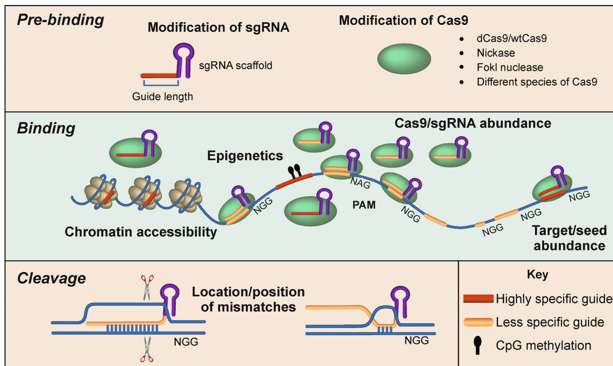
Figure 2. Factors that impact Cas9 specificity. (Top) Before Cas9 is introduced to the system, specificity can be modified by altering the architecture of the single guide RNA (sgRNA) or the Cas9 protein itself. (Middle) At the DNA level, beyond the PAM requirement for binding, closed chromatin and methylated DNA negatively impact Cas9 binding, while increased abundance of Cas9/sgRNA complexes and guide sequences in the genome positively impact Cas9 binding. (Bottom) Although Cas9 can transiently bind DNA that is complementary to only a small seed sequence in the sgRNA, only sequences with extensive complementarity to the guide will be cleaved or direct activation or silencing of targeted genes.
